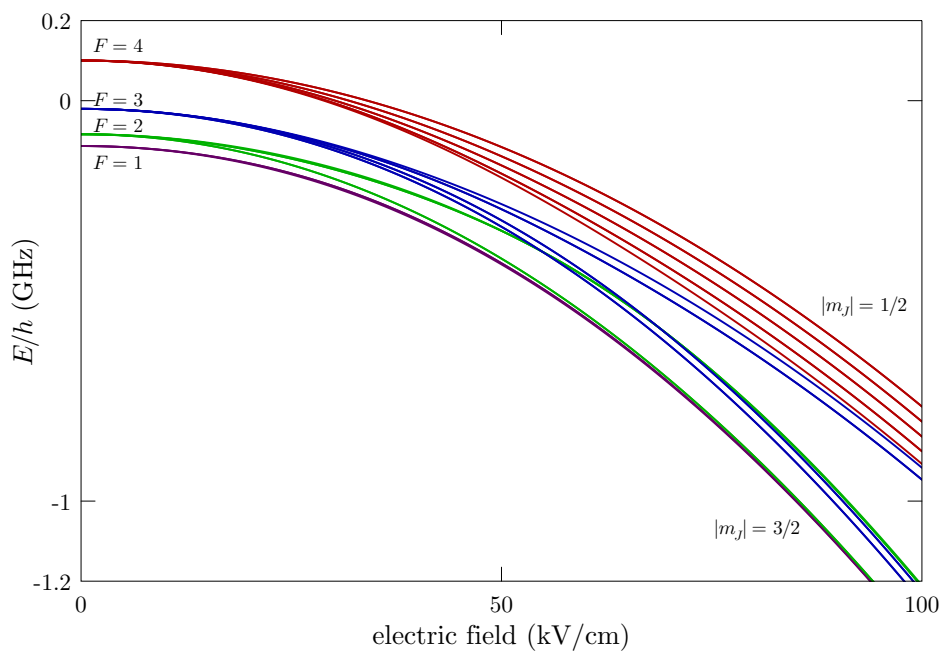
Figure 7: Rubidium 85 5^2P_{3/2} (D 2 excited) level hyperfine structure in a constant, external electric field. The levels are grouped according to the value of F in the low-field (Zeeman) regime and |m_j| in the strong-field (“electric” hyperfine Paschen-Back) regime. Levels with the same values of F and |m_F| (for a weak field) are degenerate.
