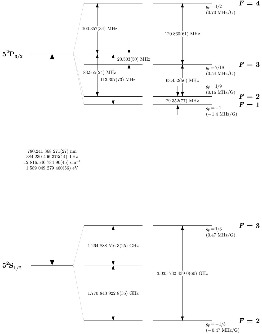
Figure 2: Rubidium 85 D_2 transition hyperfine structure, with frequency splittings between the hyperfine energy levels. The excited-state values are taken from [10, 27], and the ground-state values are from [27]. The relative hyperfine shifts are shown to scale within each hyperfine manifold (but visual spacings should not be compared between manifolds or to the optical splitting). The approximate Landé g_F -factors for each level are also given, with the corresponding Zeeman splittings between adjacent magnetic sublevels.
