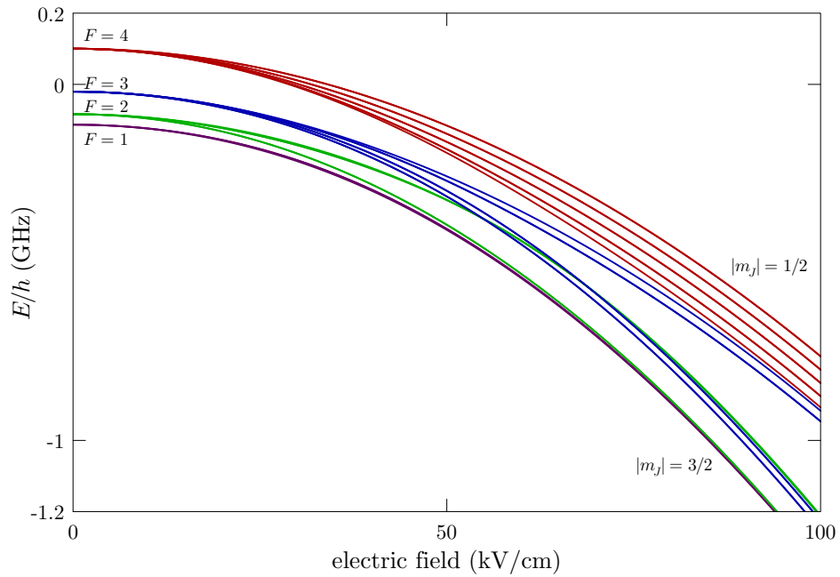
Figure 7: Rubidium 85 5^2P_{3/2} (D 2 excited) level hyperfine structure in a constant, external electric field. The levels are grouped according to the value of F in the low-field (Zeeman) regime and |m_J| in the strong-field (“electric” hyperfine Paschen-Back) regime. Levels with the same values of F and |m_F| (for a weak field) are degenerate.
