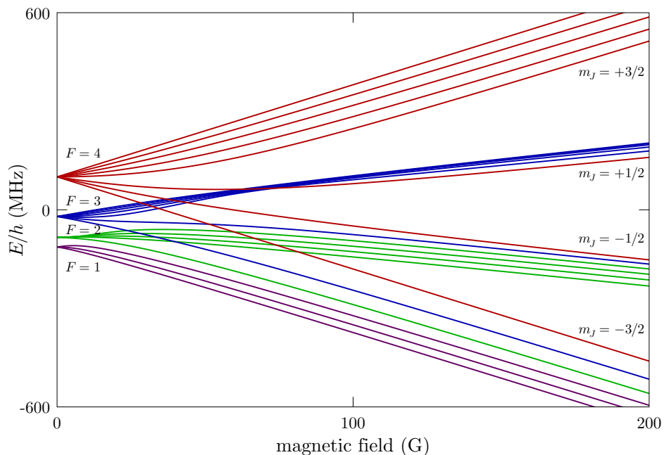
Figure 6: Rubidium 85 5^2P_{3/2} (D 2 excited) level hyperfine structure in an external magnetic field. The levels are grouped according to the value of F in the low-field (Zeeman) regime and m_j in the strong-field (hyperfine Paschen-Back) regime.
